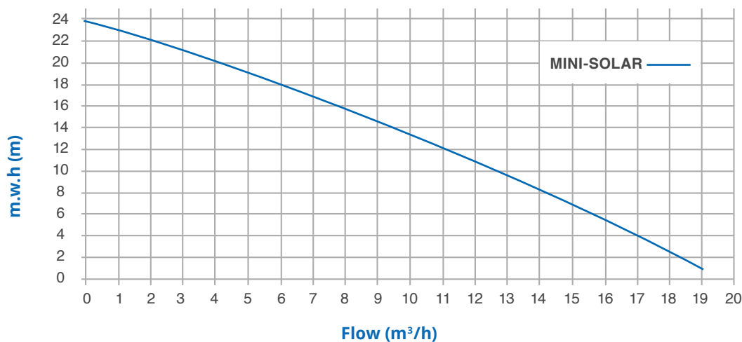
Characteristics curve
